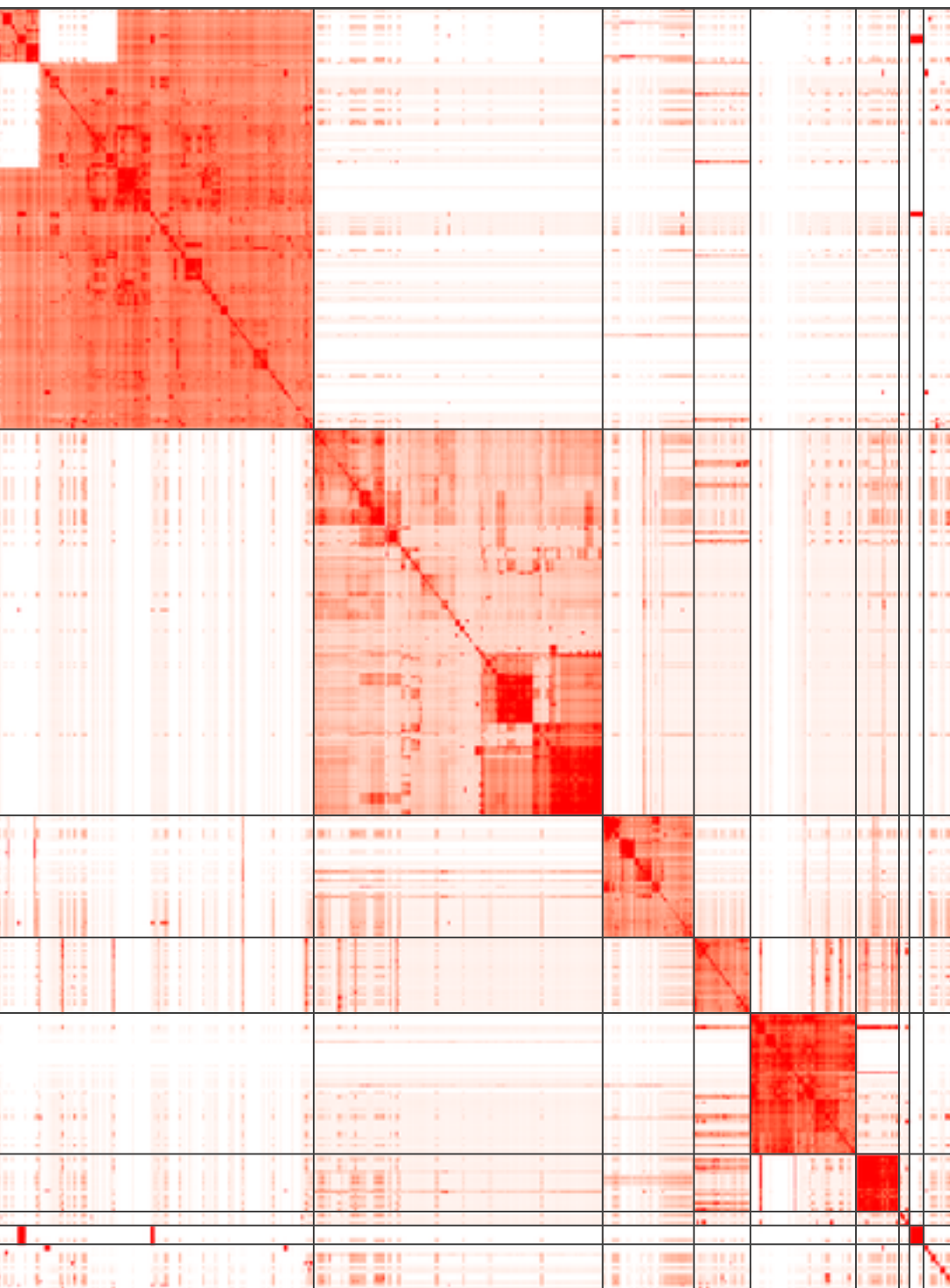
1292 GO terms clustered by 'binary_cut'
