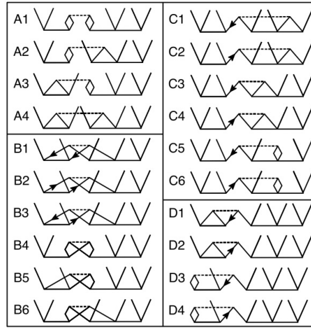
Figure 7.1: Spin-summed diagrams of \hat{T}_2\hat{T}_3 contributions to the triples residuals in CCSDT.
