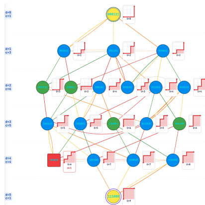
Figure 1: Original Figure 3: holography illustration for G_3(3,6) . The graph has 20 vertices; the first mismatch appears here, with mismatch ratio 1/20 .
