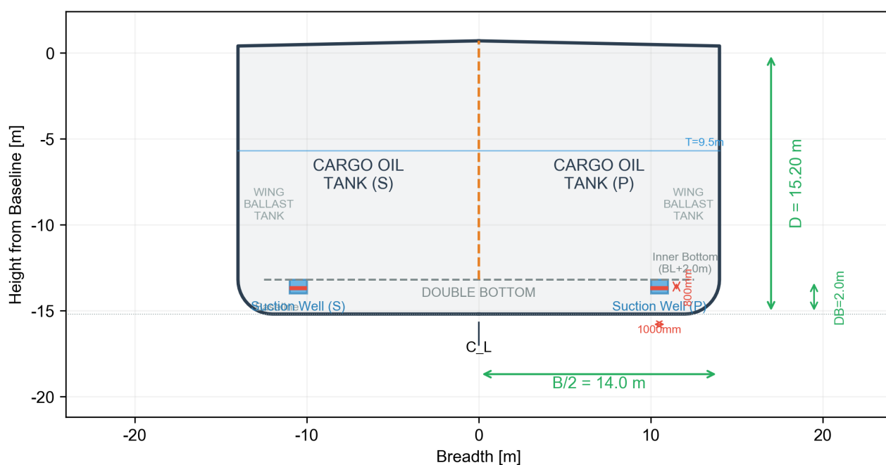
TYPICAL MIDSHIP SECTION (典型横剖面图)
