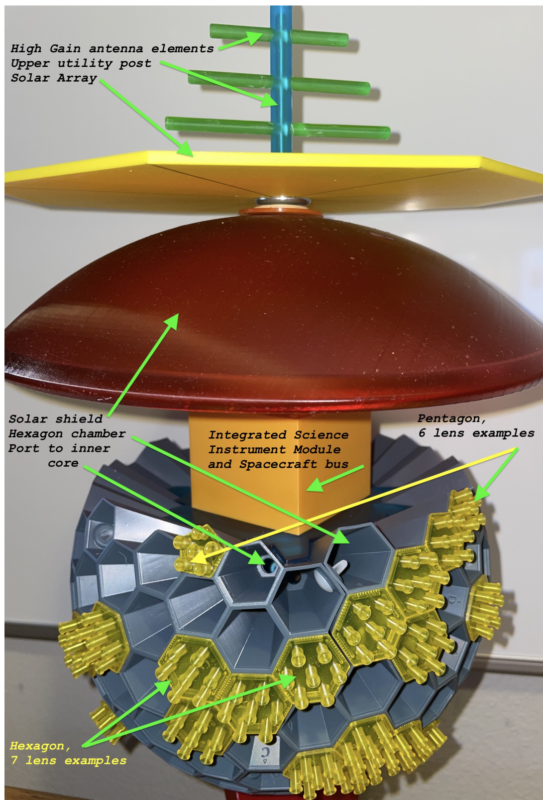
Figure B17. Photo of 3D print of prototype
