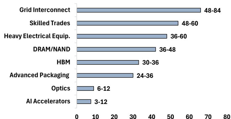
Figure 3: Lead Times in Months by Component
