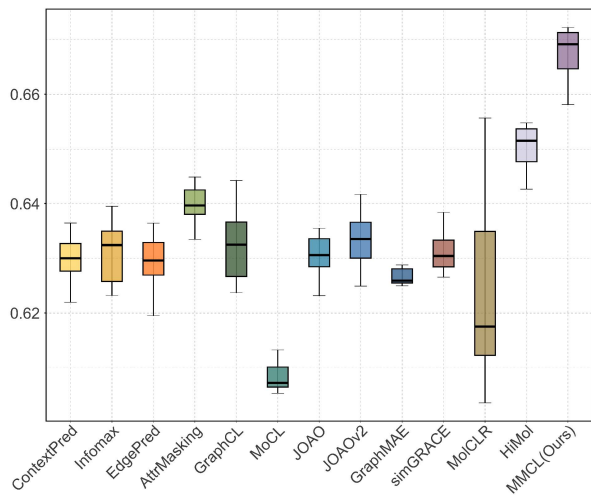
(c) Toxcast
