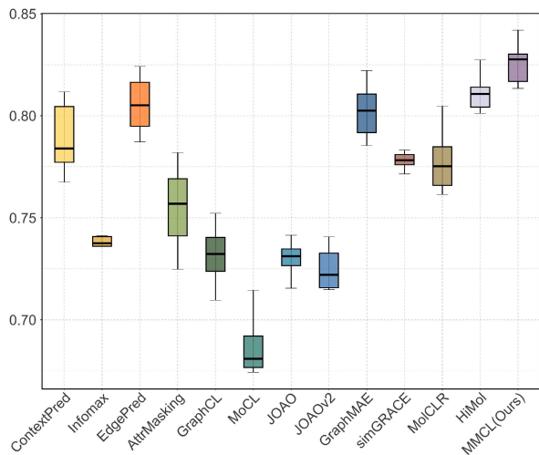
(a) BACE
