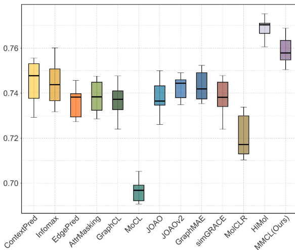
(b) Tox21
