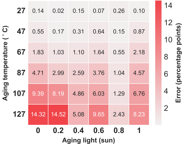
PCE retention absolute error 1000 h grouped-CV predictions
