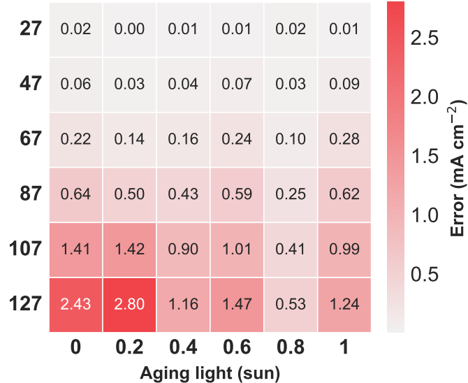
J-V current-density absolute error 1000 h grouped-CV predictions
