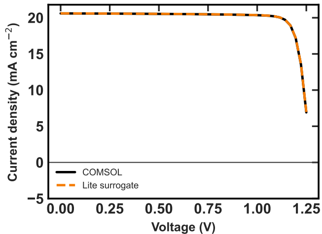
1 sun, 127 °C, 1000 h
