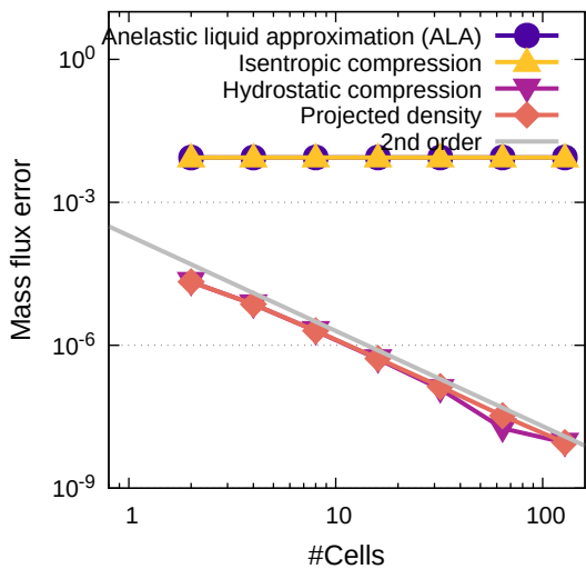
Mass flux error: Sub-adiabatic temperature
