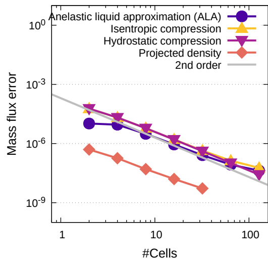
Mass flux error: Adiabatic temperature
