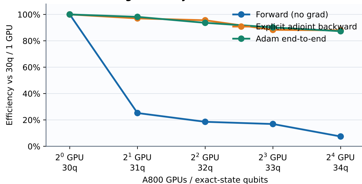
b Weak-scaling efficiency
