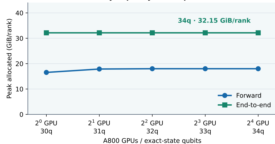
c Constant-memory capacity envelope
