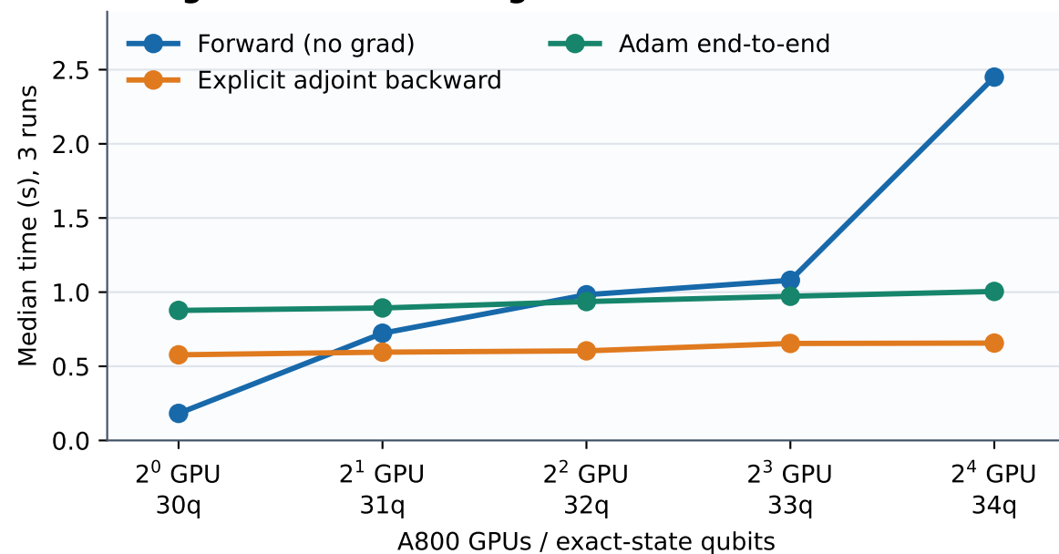
a High-load weak scaling · measured time
