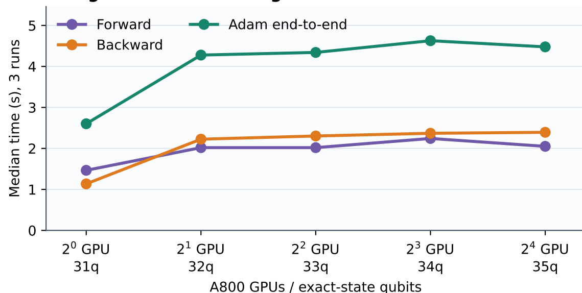
a High-load weak scaling · measured time
