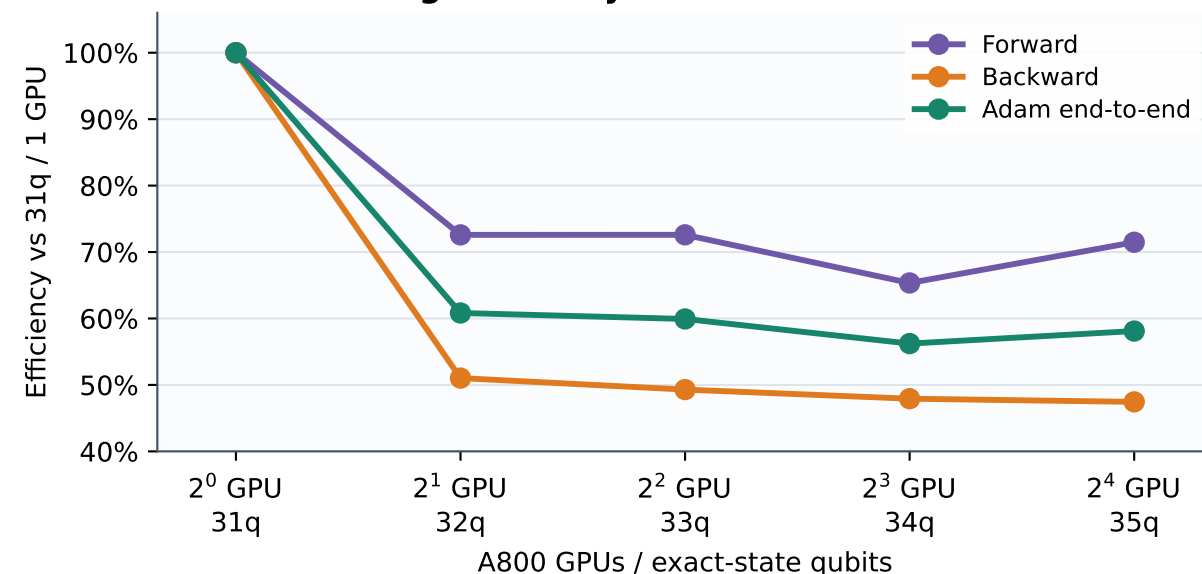
b Weak-scaling efficiency
