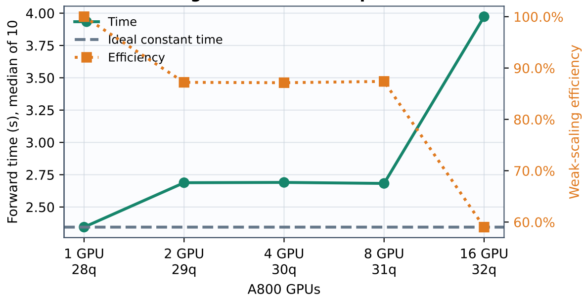
c Weak scaling · constant 2^{28} amplitudes/GPU
