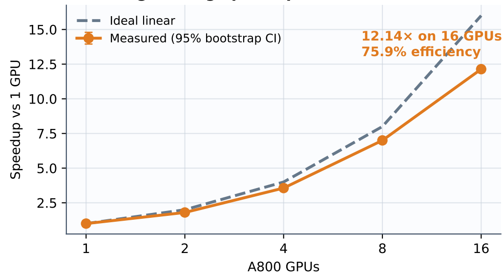
b Strong-scaling speedup
