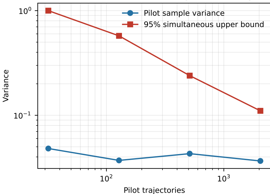
(a) Statistical evidence tightens slowly
