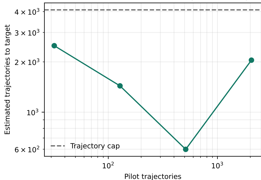
(b) Conservative time-to-target planning
