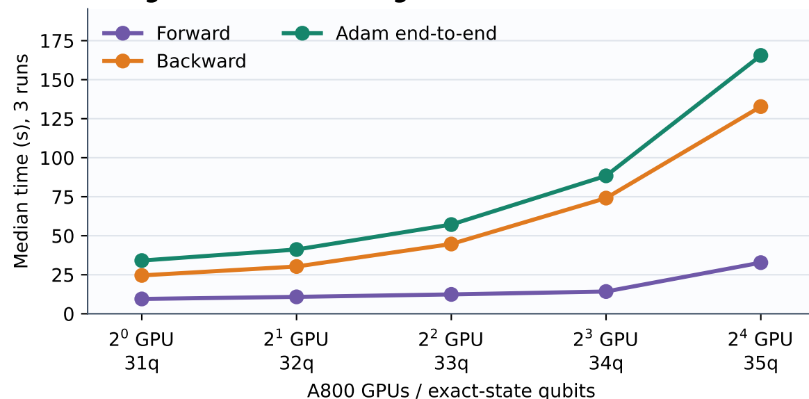
a High-load weak scaling · measured time
