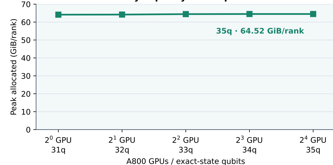
c Constant-memory capacity envelope
