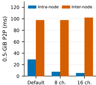
a Transport latency
