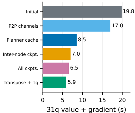
c 16-GPU optimization sequence
