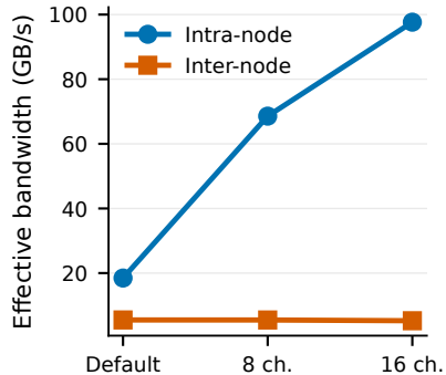
b Effective P2P bandwidth
