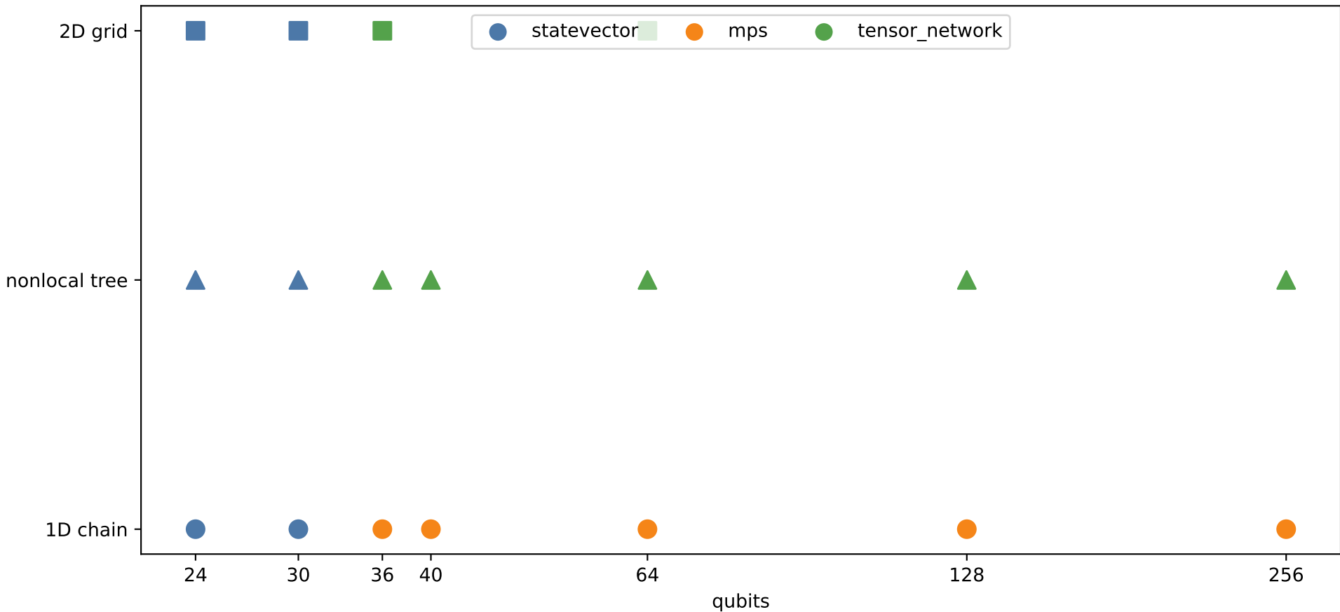
Gradient backend phase diagram: expectation, complex128
