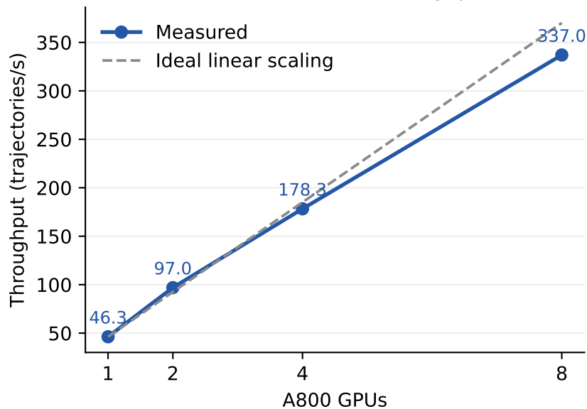
(a) Fixed-workload throughput
