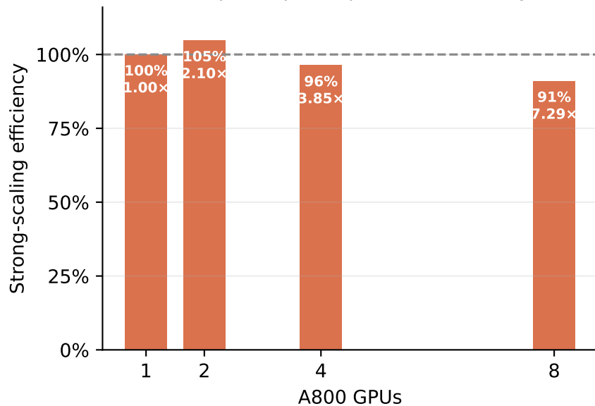
(b) Speedup and parallel efficiency
