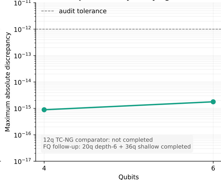
c complex128 trajectory agreement
