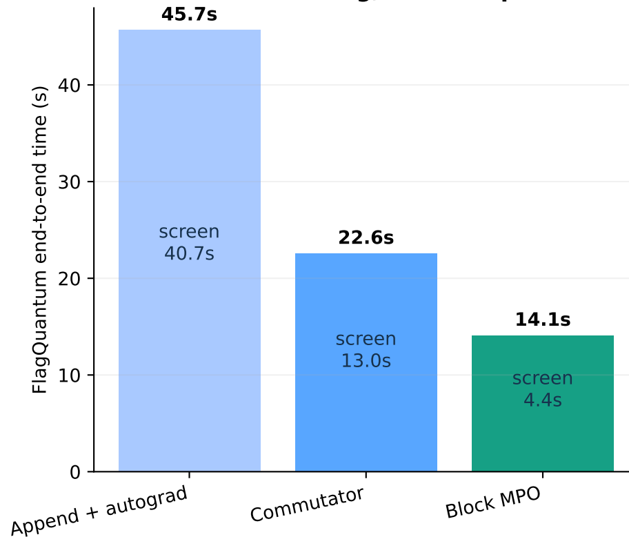
b Exact screening, same 12q result
