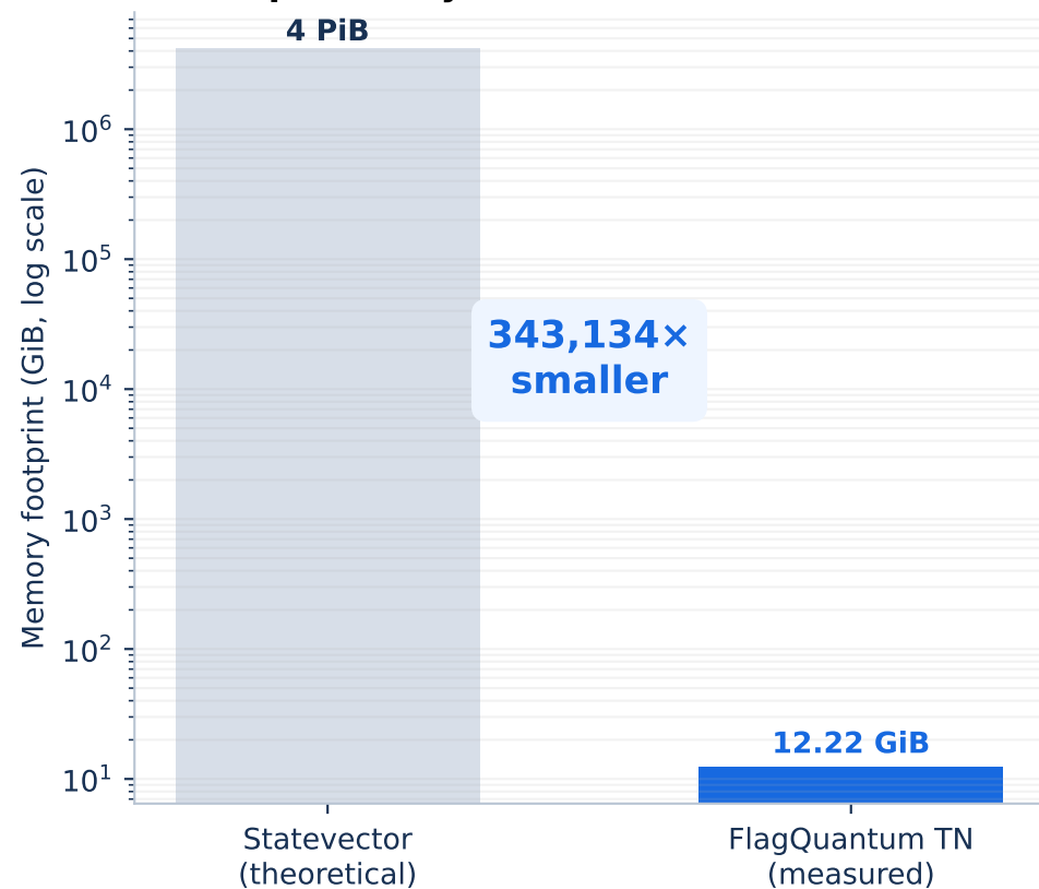
a 48 qubits beyond statevectors
