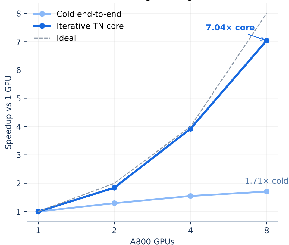
b Real 16-slice strong scaling
