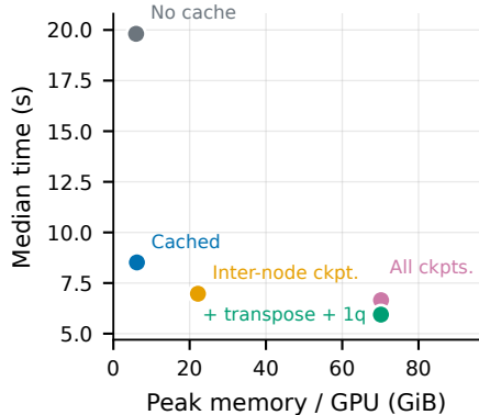
c 16-GPU time-memory Pareto
