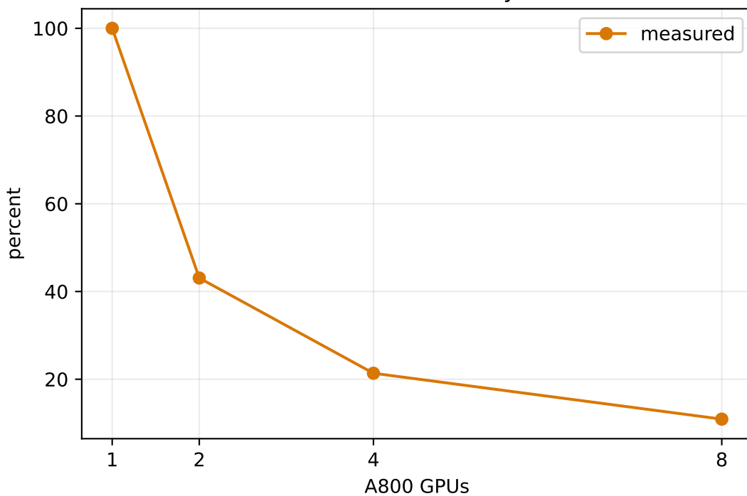
Parallel efficiency
