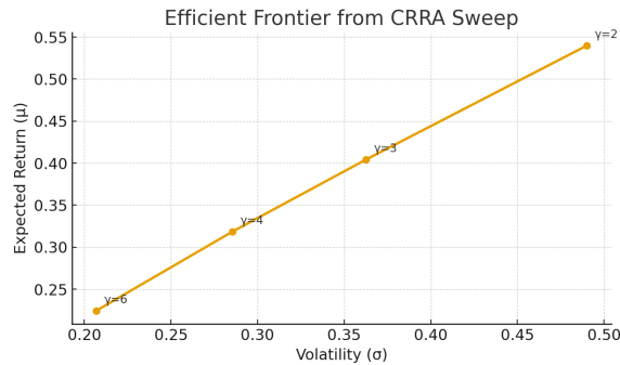
Figure 9: Efficient frontier generated from the CRRA sweep ( \gamma = 2, 3, 4, 6 ). Each point represents the optimal portfolio at a given risk aversion level, moving down and left along the frontier as \gamma increases.
