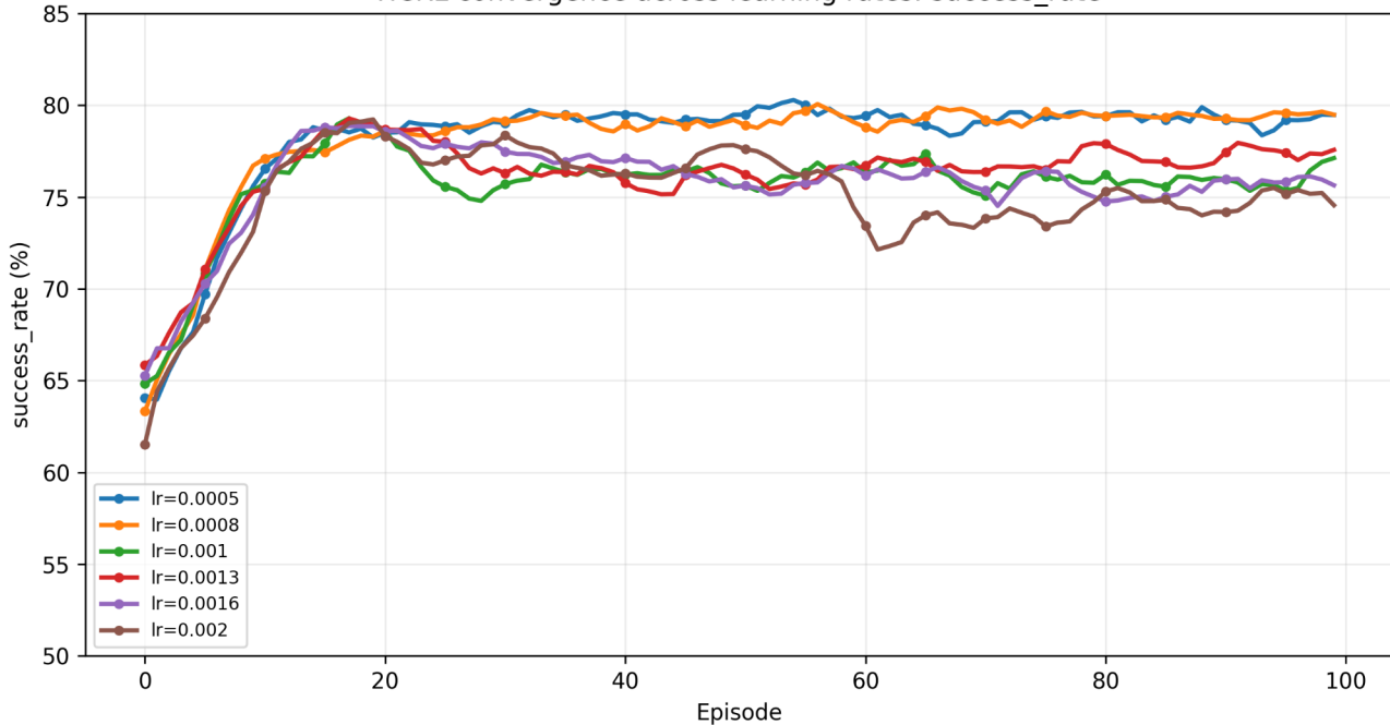
HCRL convergence across learning rates: success_rate
