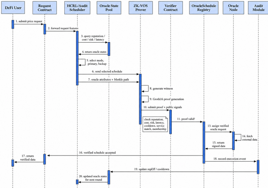
ZK-VOS proof generation and verification workflow
