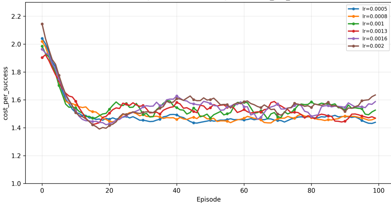
HCRL convergence across learning rates: cost_per_success
