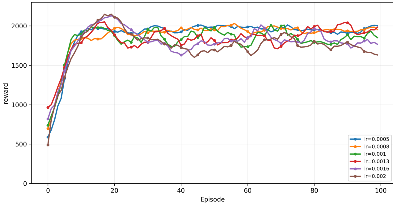
HCRL convergence across learning rates: reward
