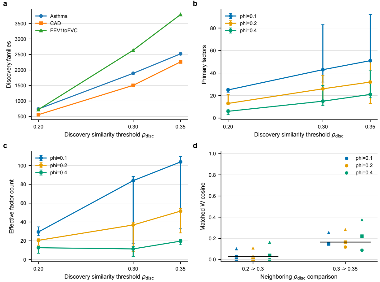
Figure 1: Tuning the discovery similarity threshold. Panels show discovery family counts, primary factor counts, effective factor counts, and neighboring-threshold matched- W cosine summaries across large Asthma, CAD, and FEV1toFVC panels.
