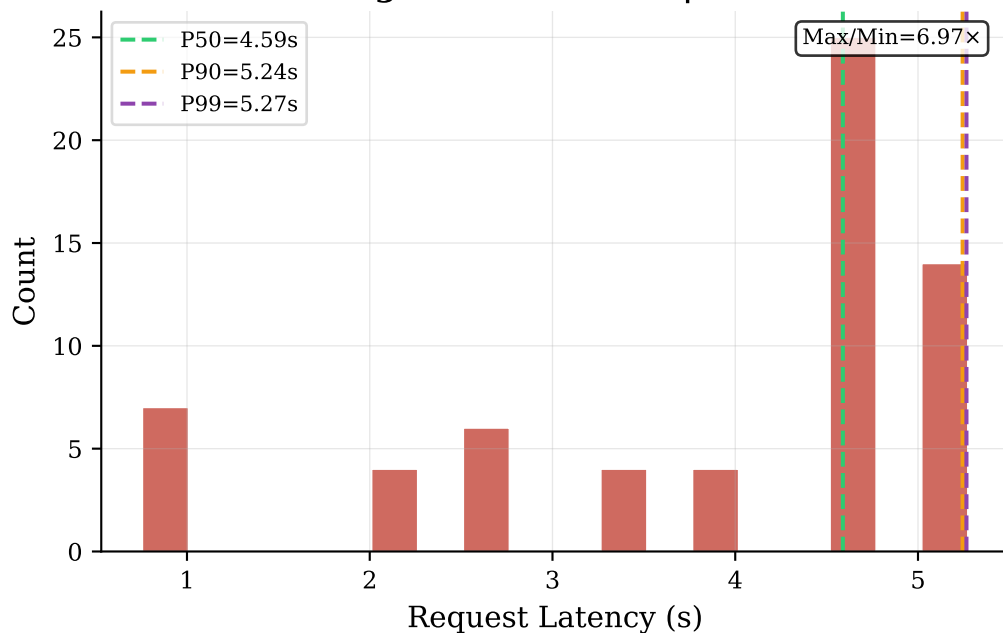
Block Length = 64 tokens | CV = 0.370
