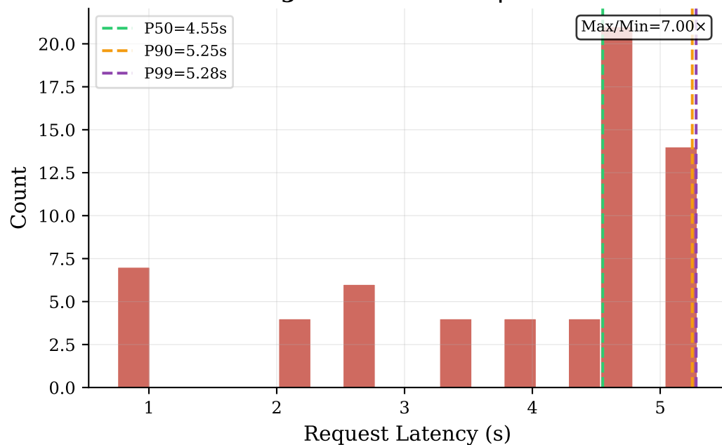
Block Length = 64 tokens | CV = 0.370
