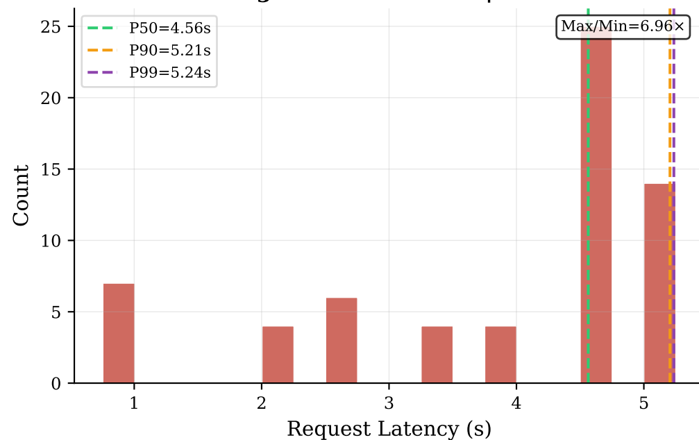
Block Length = 128 tokens | CV = 0.368
