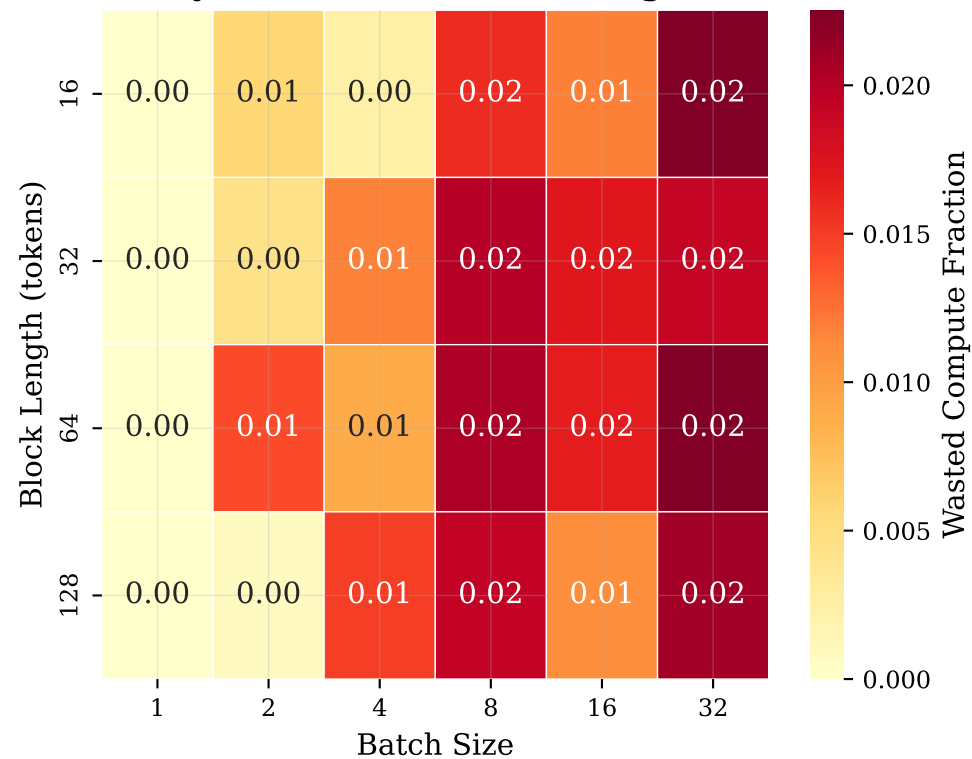
(B1a) Synchronous Waste Fraction by Batch Size × Block Length
