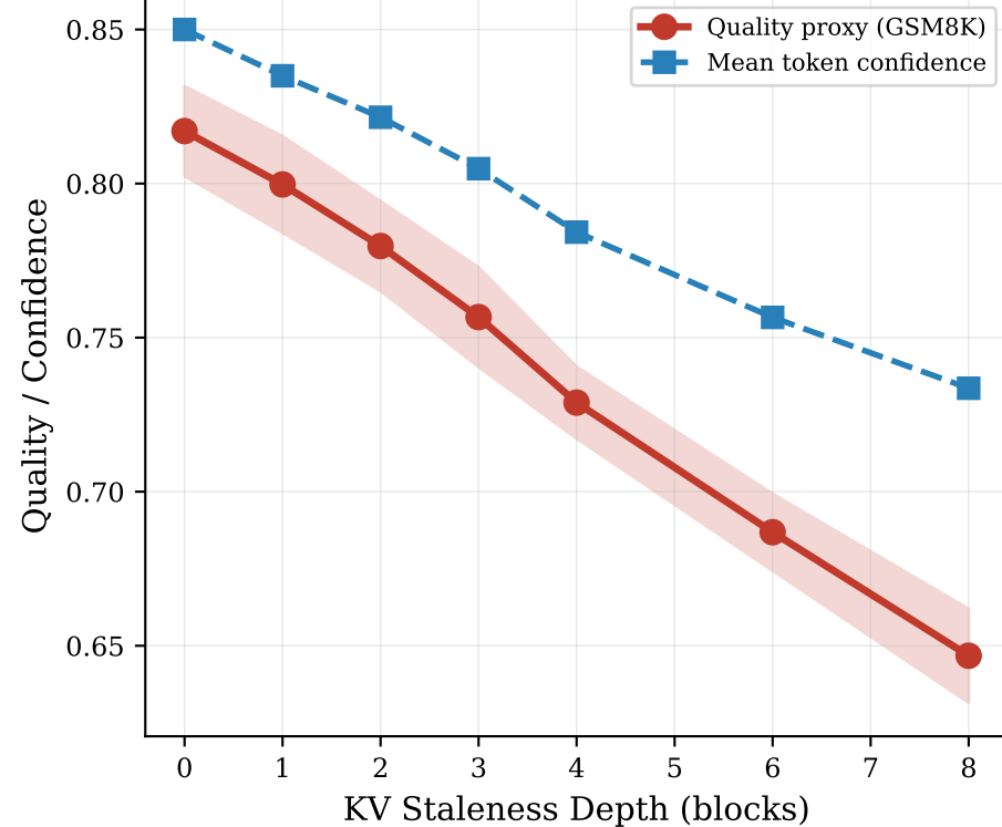
(F1a) Quality Degradation vs KV Staleness
