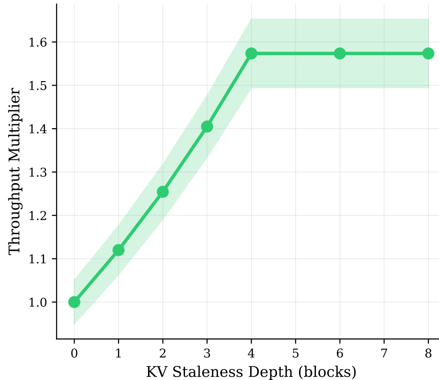
(F1b) Throughput Gain from Pipelined Decoding
