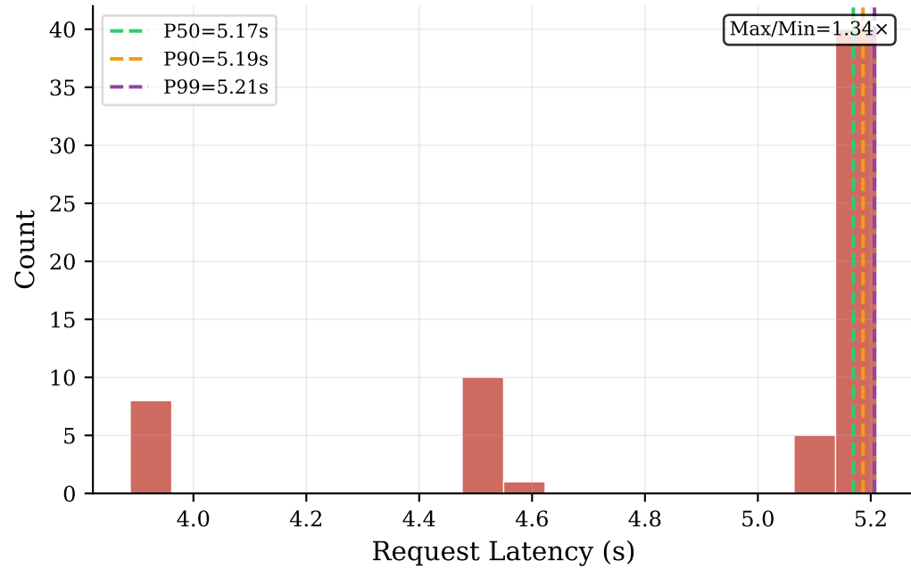
Block Length = 128 tokens | CV = 0.091
