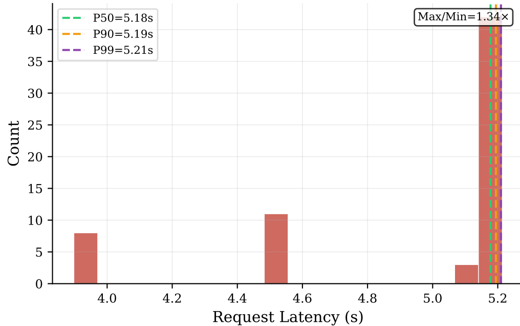
Block Length = 64 tokens | CV = 0.092
