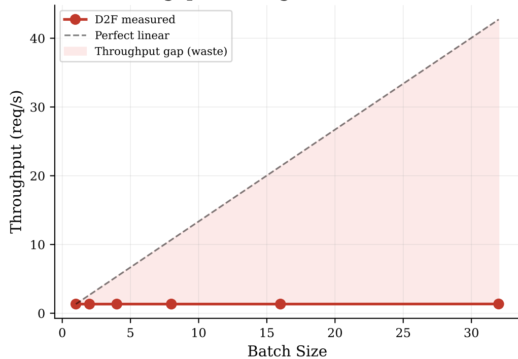
Throughput Scaling (Block=32 tokens)
