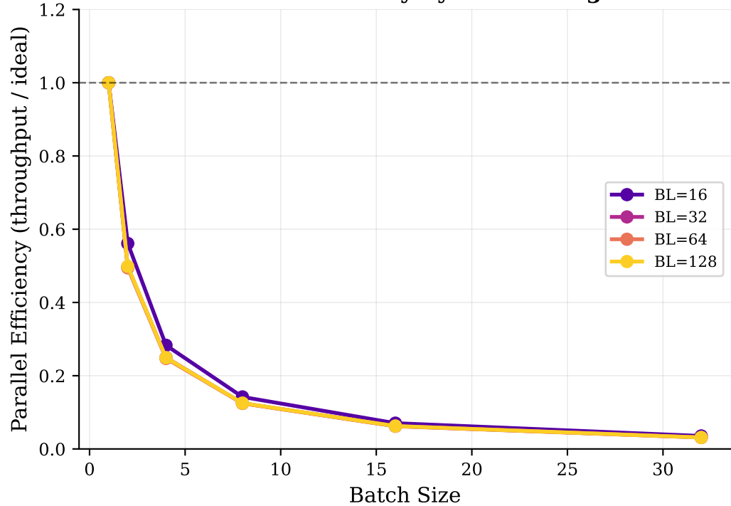
Parallel Efficiency by Block Length
