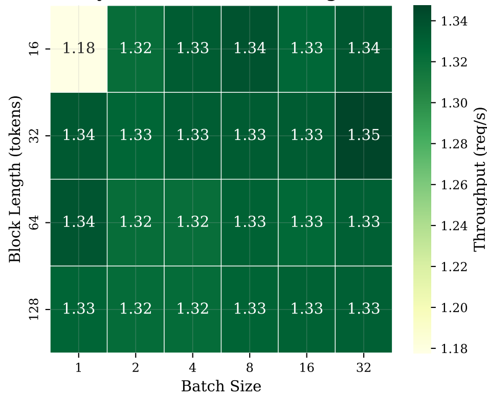
(B1b) Throughput (req/s) by Batch Size × Block Length
