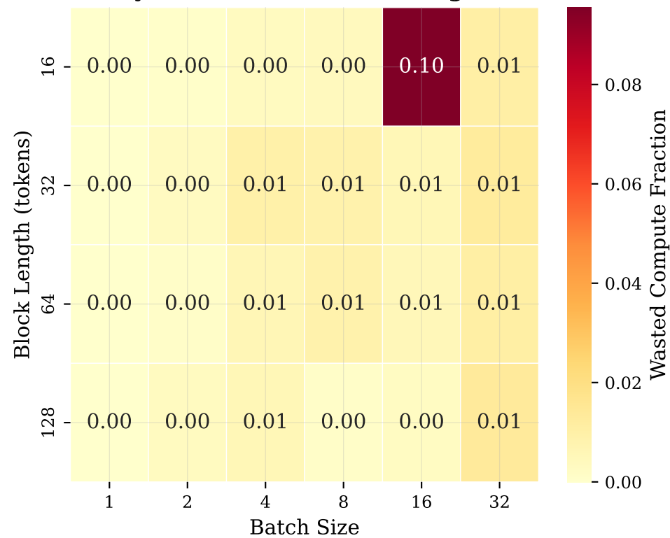
(B1a) Synchronous Waste Fraction by Batch Size × Block Length
