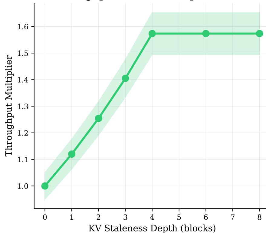
(F1b) Throughput Gain from Pipelined Decoding
