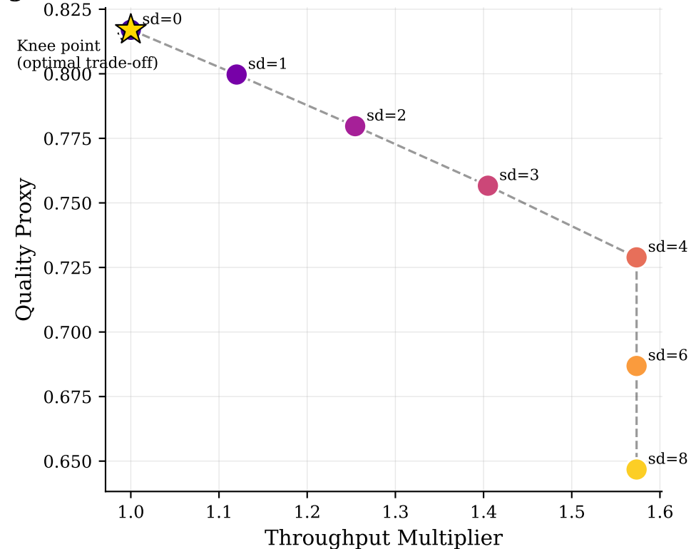
(F1c) Quality-Throughput Pareto KV Staleness Trade-off
