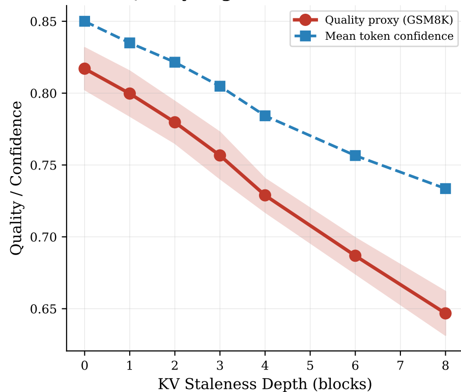
(F1a) Quality Degradation vs KV Staleness
