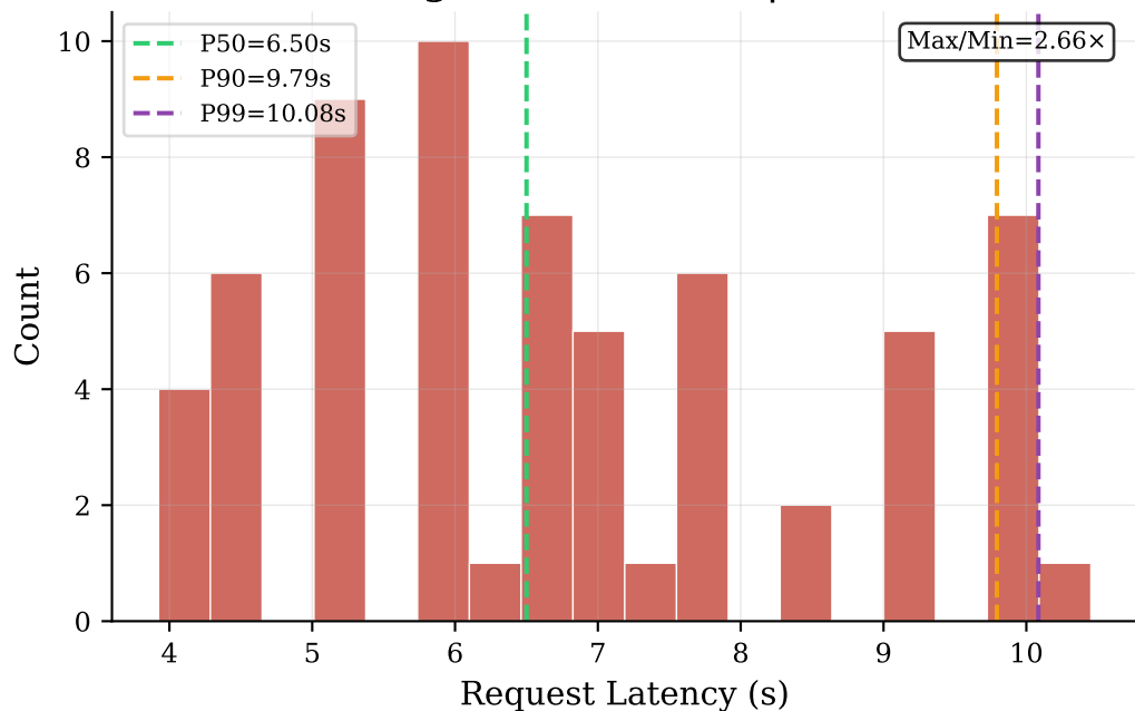
Block Length = 64 tokens | CV = 0.270
