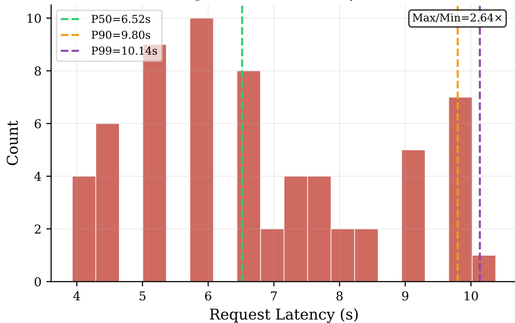
Block Length = 128 tokens | CV = 0.271
