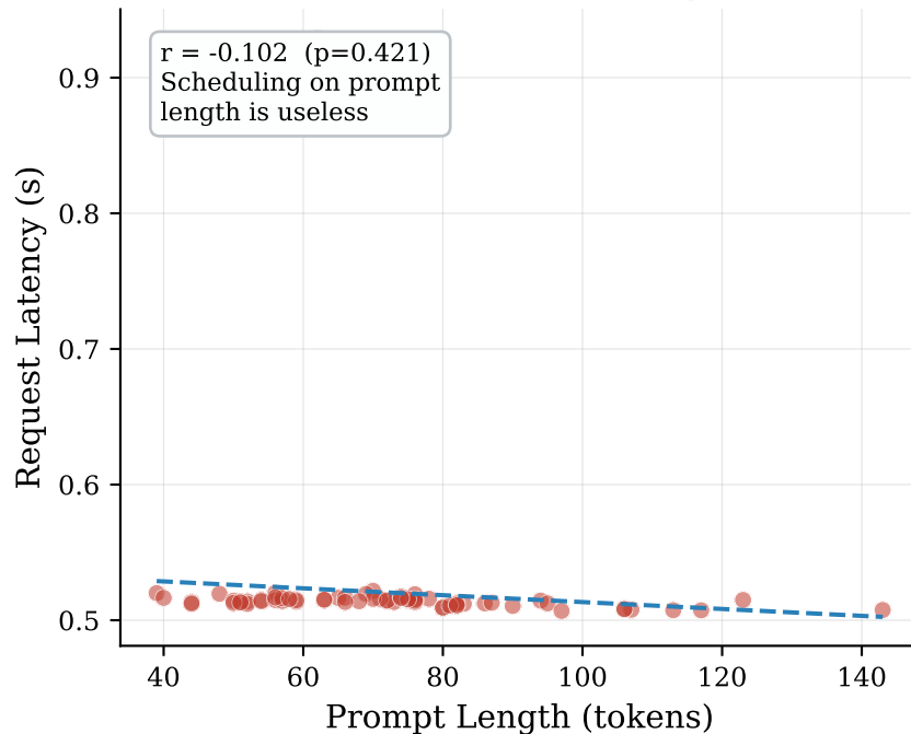
Prompt Length vs Latency | r = -0.102
