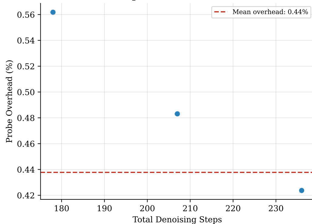
Probe Overhead vs Request Difficulty Harder requests have lower overhead
