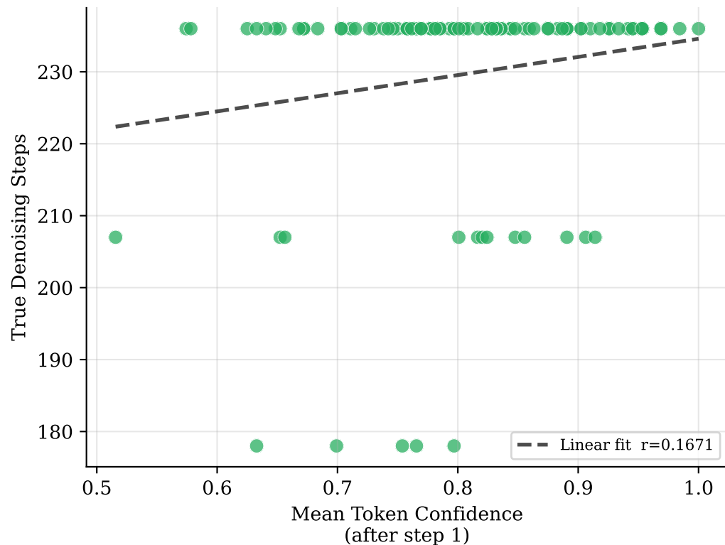
Best Probe Signal vs True Steps R^2=0.0279
