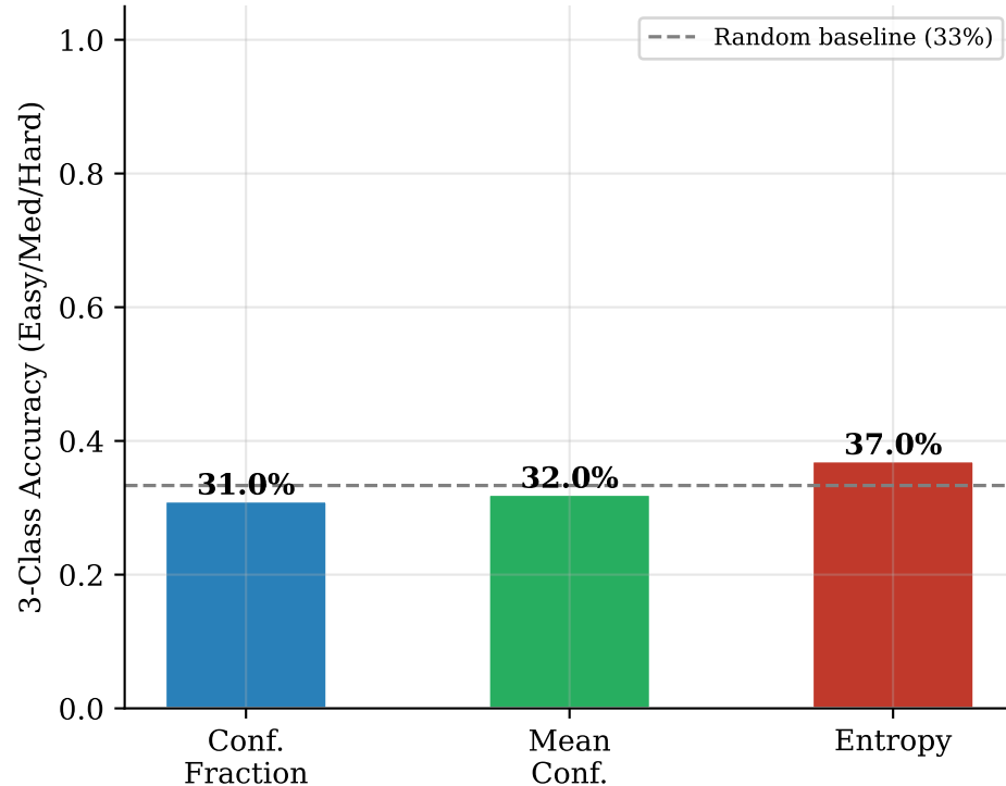
Classification Accuracy by Probe Signal
