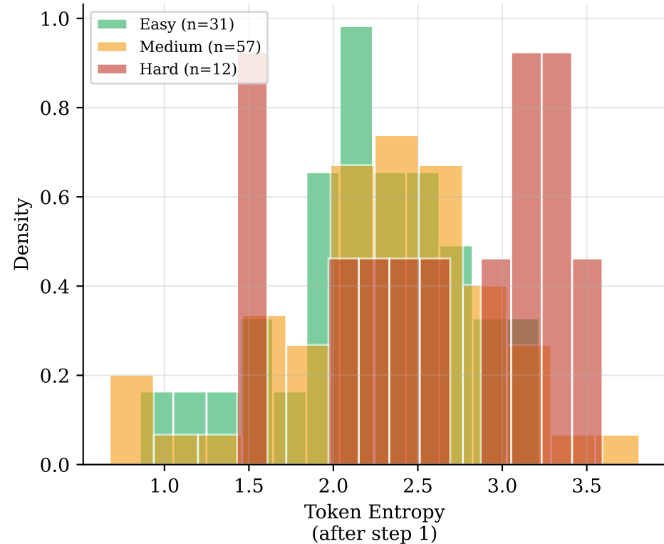
Best Signal: entropy by Difficulty Tier
