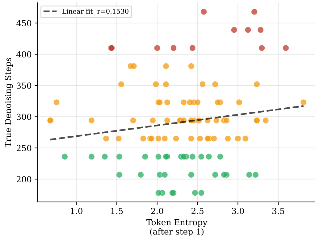
Best Probe Signal vs True Steps R^2=0.0234
