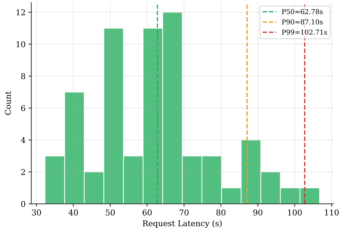
Slot-Based CV=0.2685
