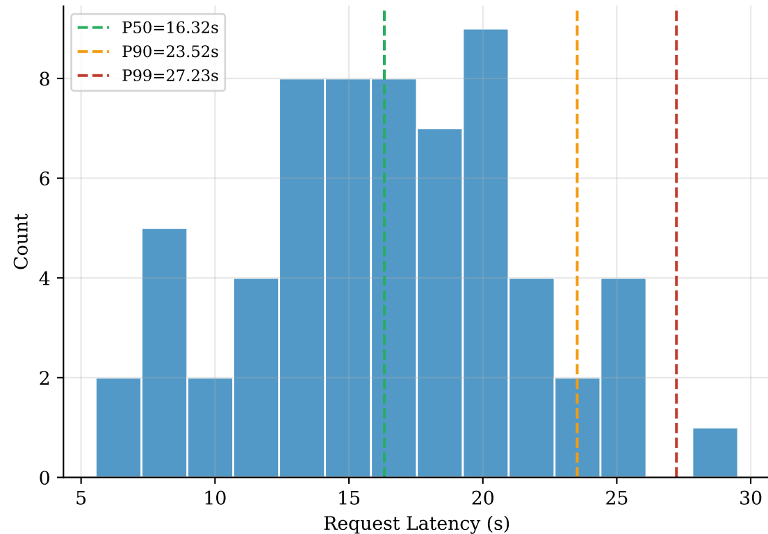
FCFS CV=0.3173
