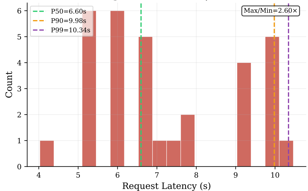
Block Length = 128 tokens | CV = 0.259
