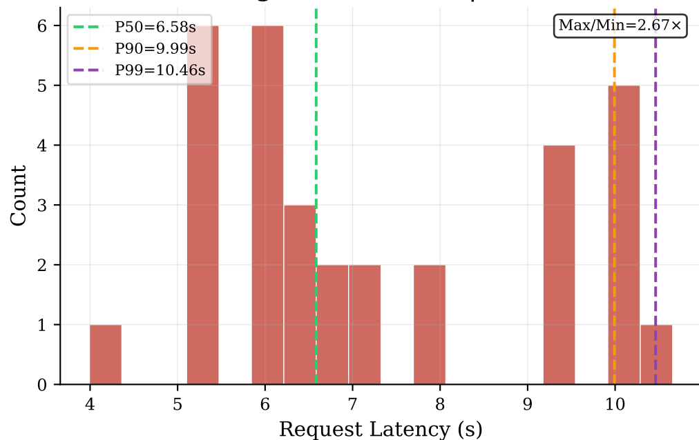
Block Length = 64 tokens | CV = 0.259
