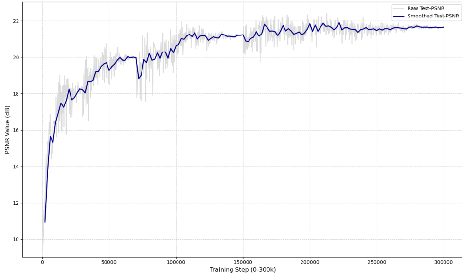
Figure 6: PSNR of denoised images on the test dataset across training steps for 1-NFE denoising.
