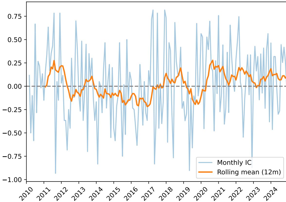
Cross-Sectional IC (mean=0.019, t \approx 0.62 )
