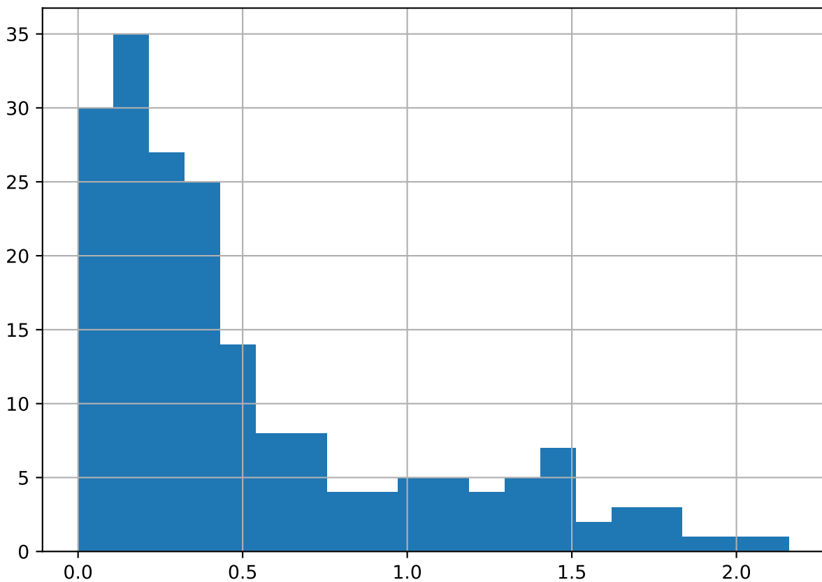
Turnover Distribution (mean=0.52, median=0.33)
