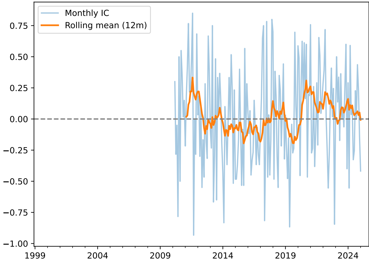
Cross-Sectional IC (mean=0.022, t \approx 0.73 )
