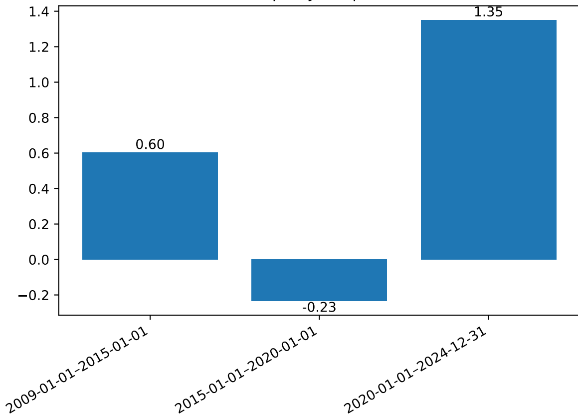
Sharpe by Subperiod
