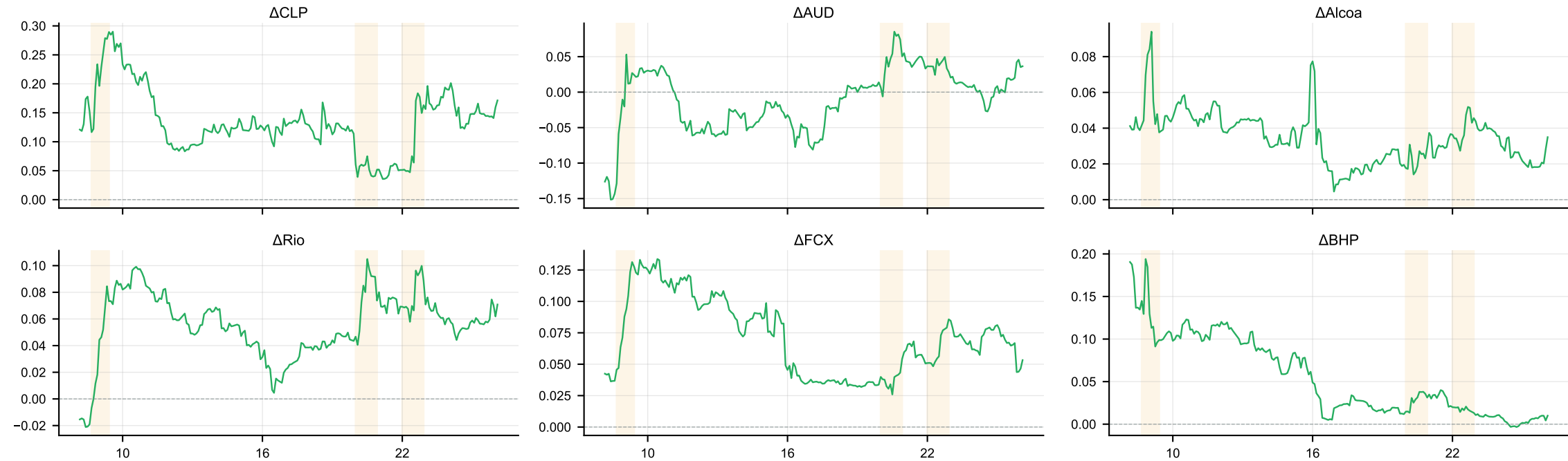
Figure A3c: DMA Time-Varying Coefficients \beta(\text{DMA}) — FX & Mining Stock Variables (March 2008 – February 2026)
