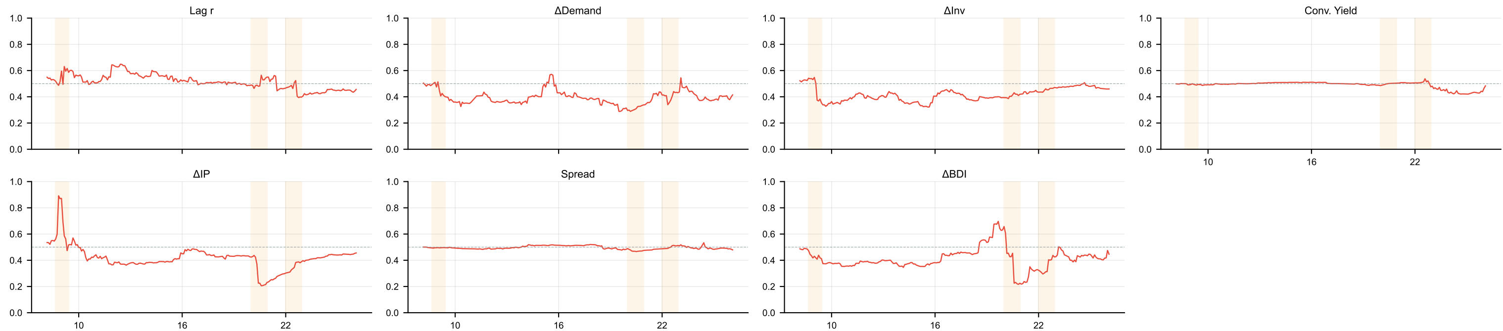
Figure A2a: Posterior Inclusion Probabilities — Fundamental Variables (March 2008 – February 2026)
