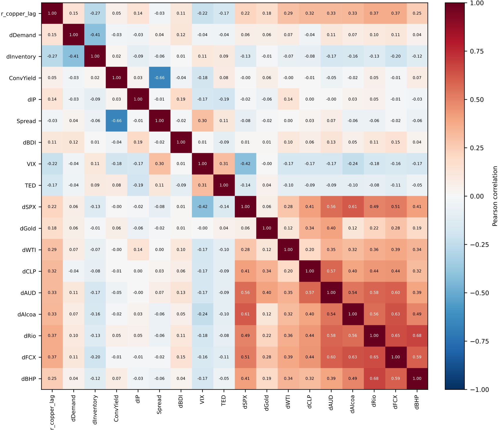
Predictor Correlation Matrix (March 1998 - February 2026)
