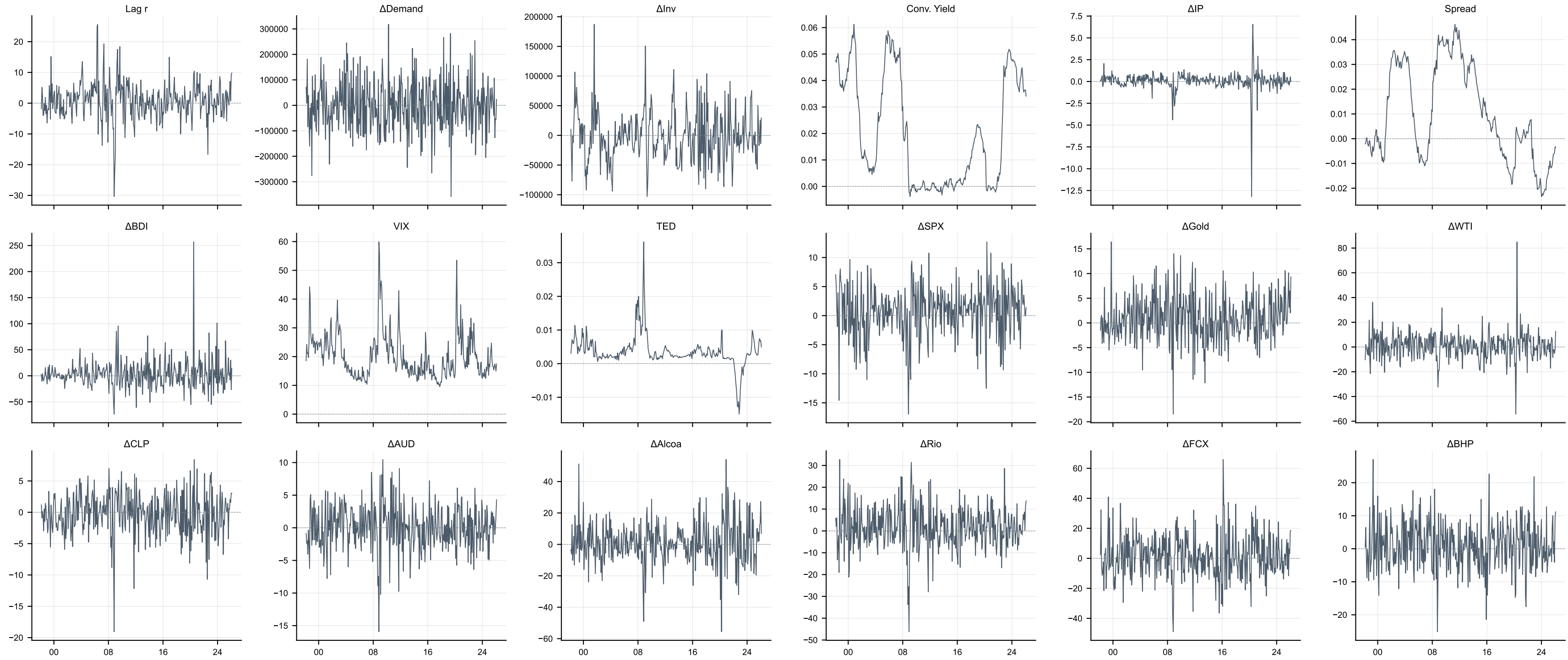
Figure A1: Time Series of All 18 Predictor Variables (March 1998 – February 2026)
