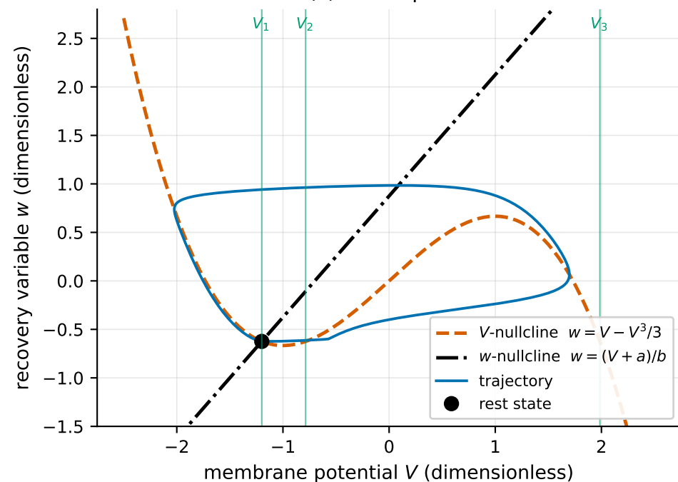
(c) Phase plane
