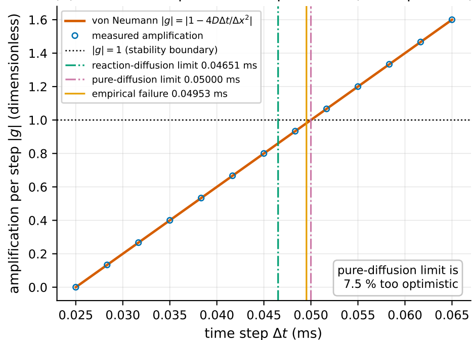
(d) Measured vs predicted amplification (linear problem)
